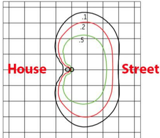
Grid Distance in Units of Mounting Height at 16' Initial Footcandle Values at Grade
